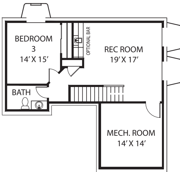
BASEMENT LEVEL
